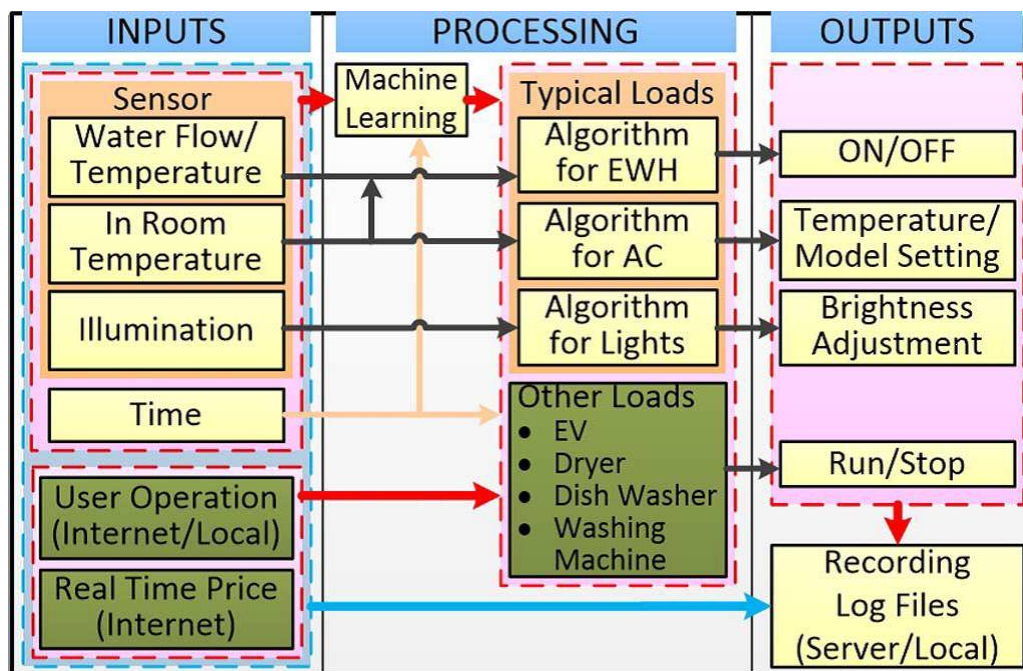
Figure 2: Schematic design of SHEMS (user end)
