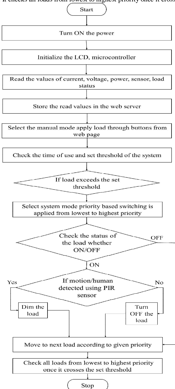
Figure 3: Flowchart of proposed system
